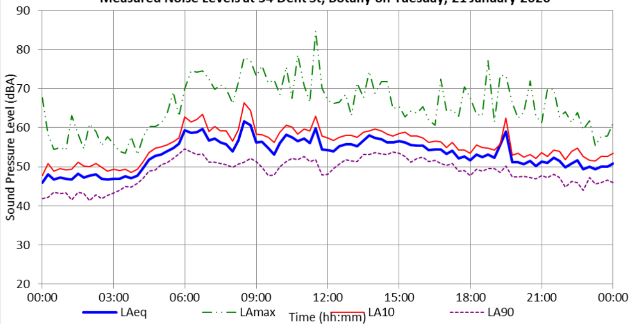
Measured Noise Levels at 34 Dent St, Botany on Tuesday, 21 January 2020
