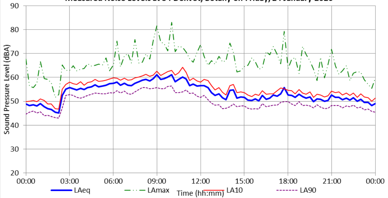
Measured Noise Levels at 34 Dent St, Botany on Friday, 24 January 2020
