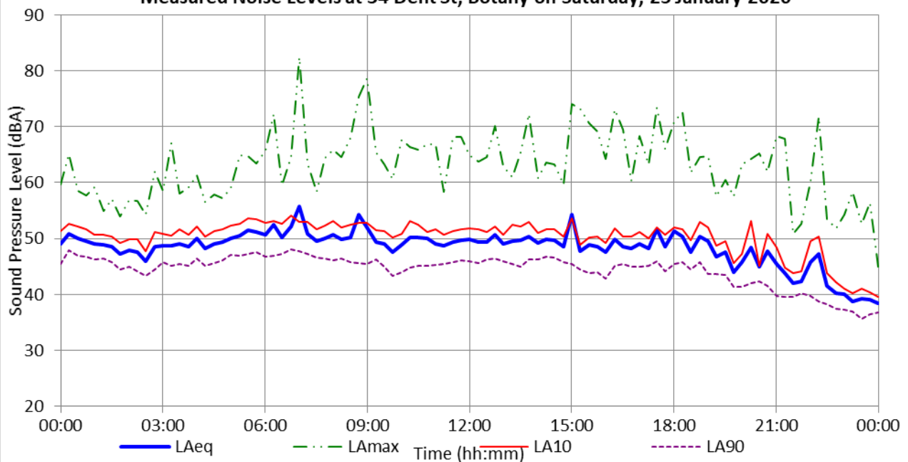
Measured Noise Levels at 34 Dent St, Botany on Saturday, 25 January 2020
