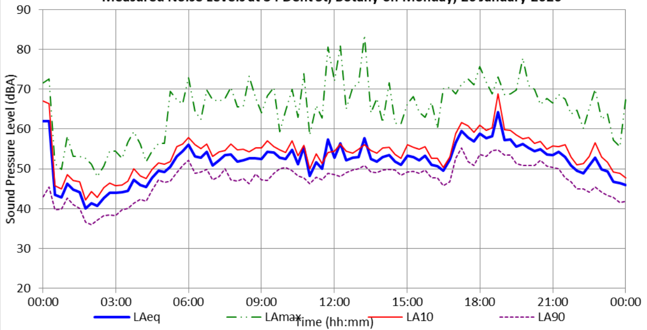
Measured Noise Levels at 34 Dent St, Botany on Monday, 20 January 2020
