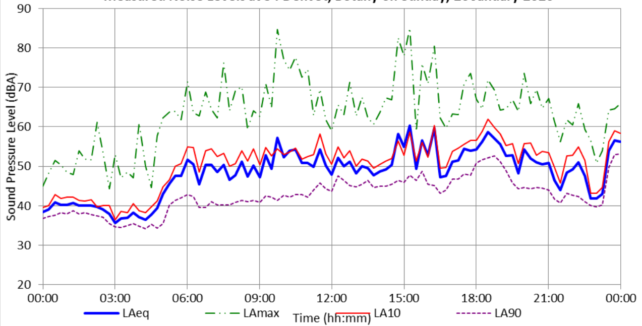
Measured Noise Levels at 34 Dent St, Botany on Sunday, 26 January 2020
