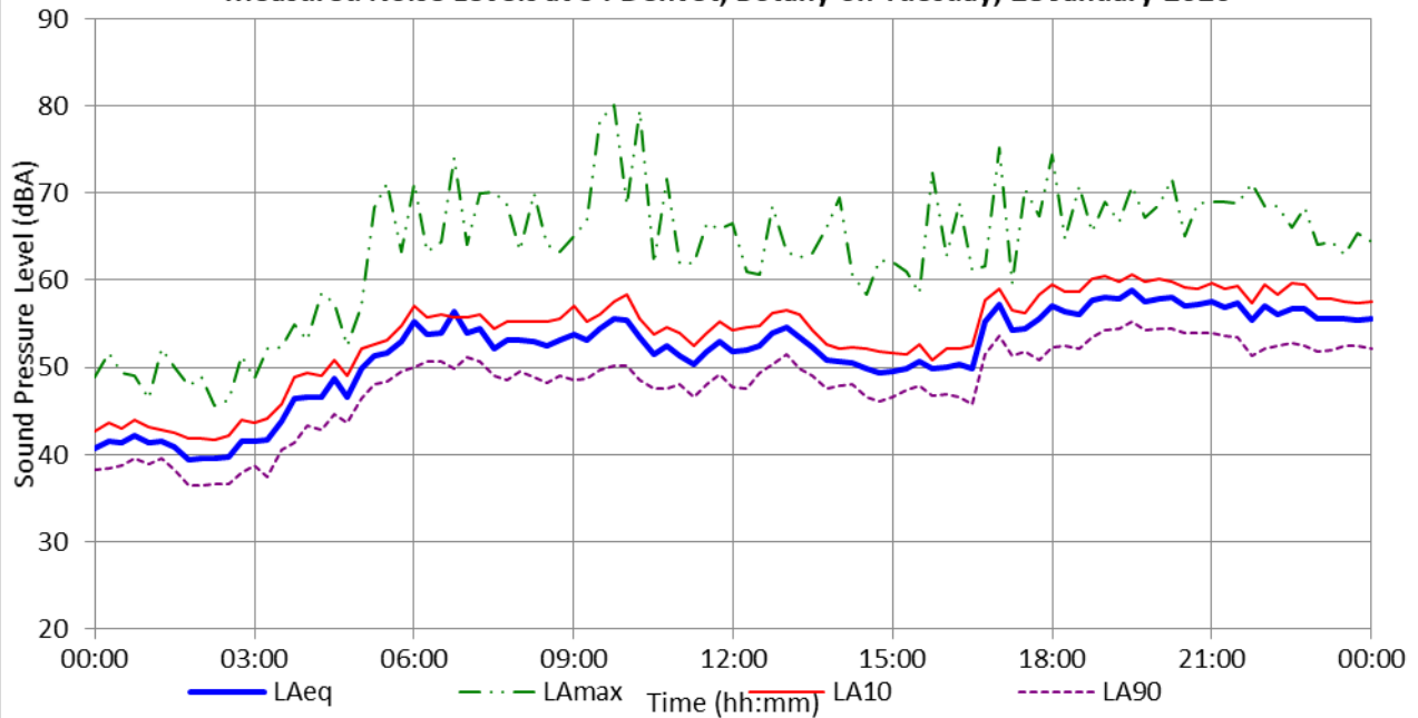
Measured Noise Levels at 34 Dent St, Botany on Tuesday, 28 January 2020
