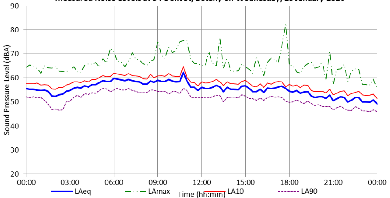
Measured Noise Levels at 34 Dent St, Botany on Wednesday, 29 January 2020
