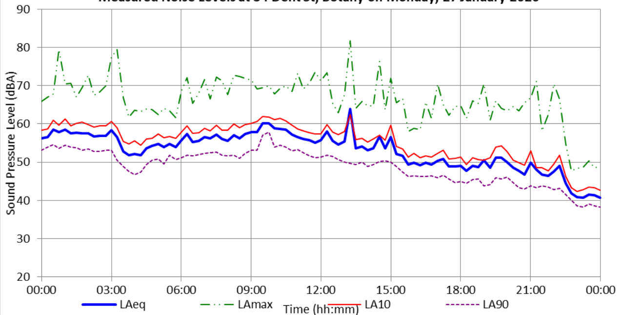
Measured Noise Levels at 34 Dent St, Botany on Monday, 27 January 2020
